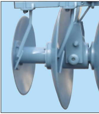
Dischetto coprisolco (optional) Furrow covering disc (optional)
